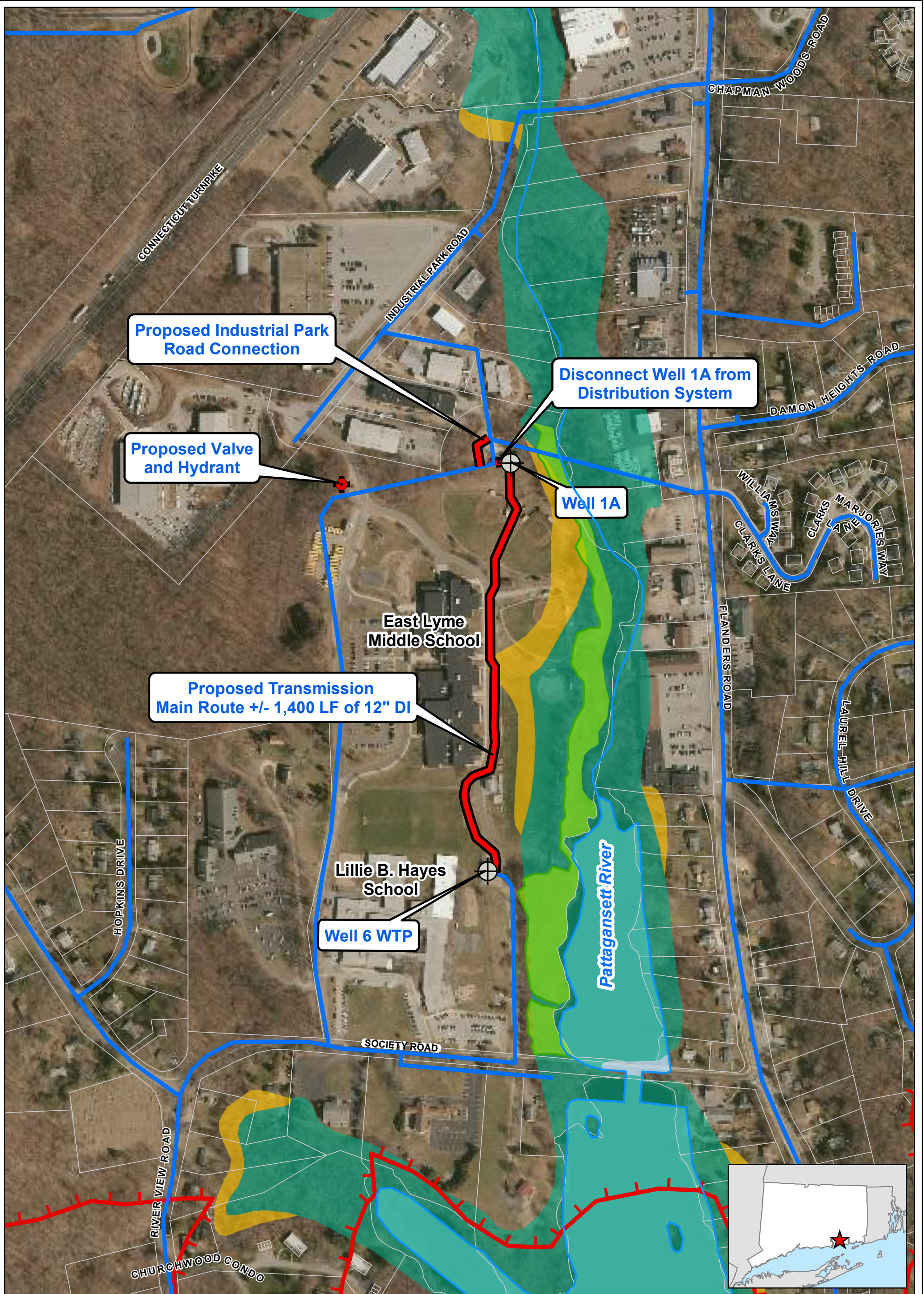
FIGURE 2 PROPOSED WELL 1A RAW WATER TRANSMISSION MAIN
