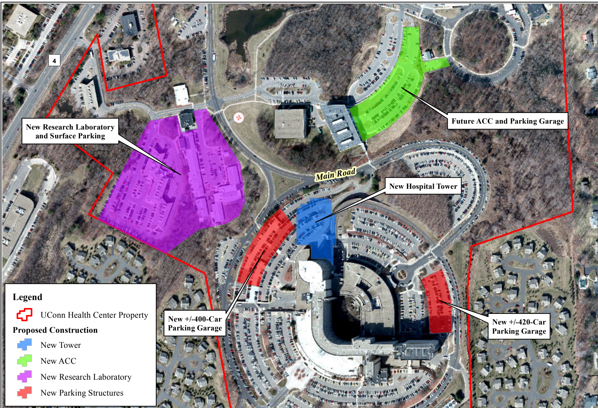
Figure ES-1: Proposed Construction Areas
