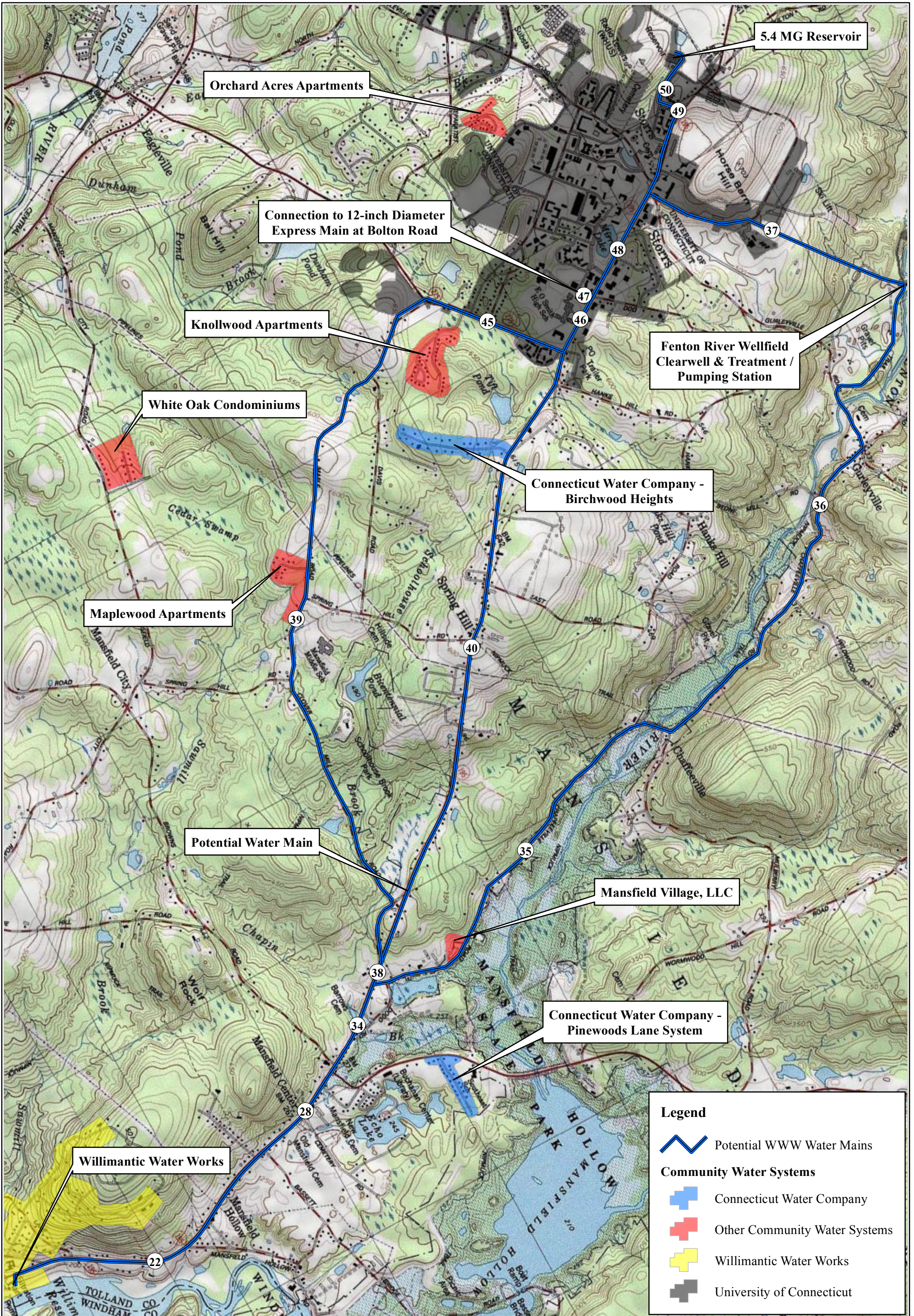
Figure 3.6-1: WWW Interconnection Alternative
