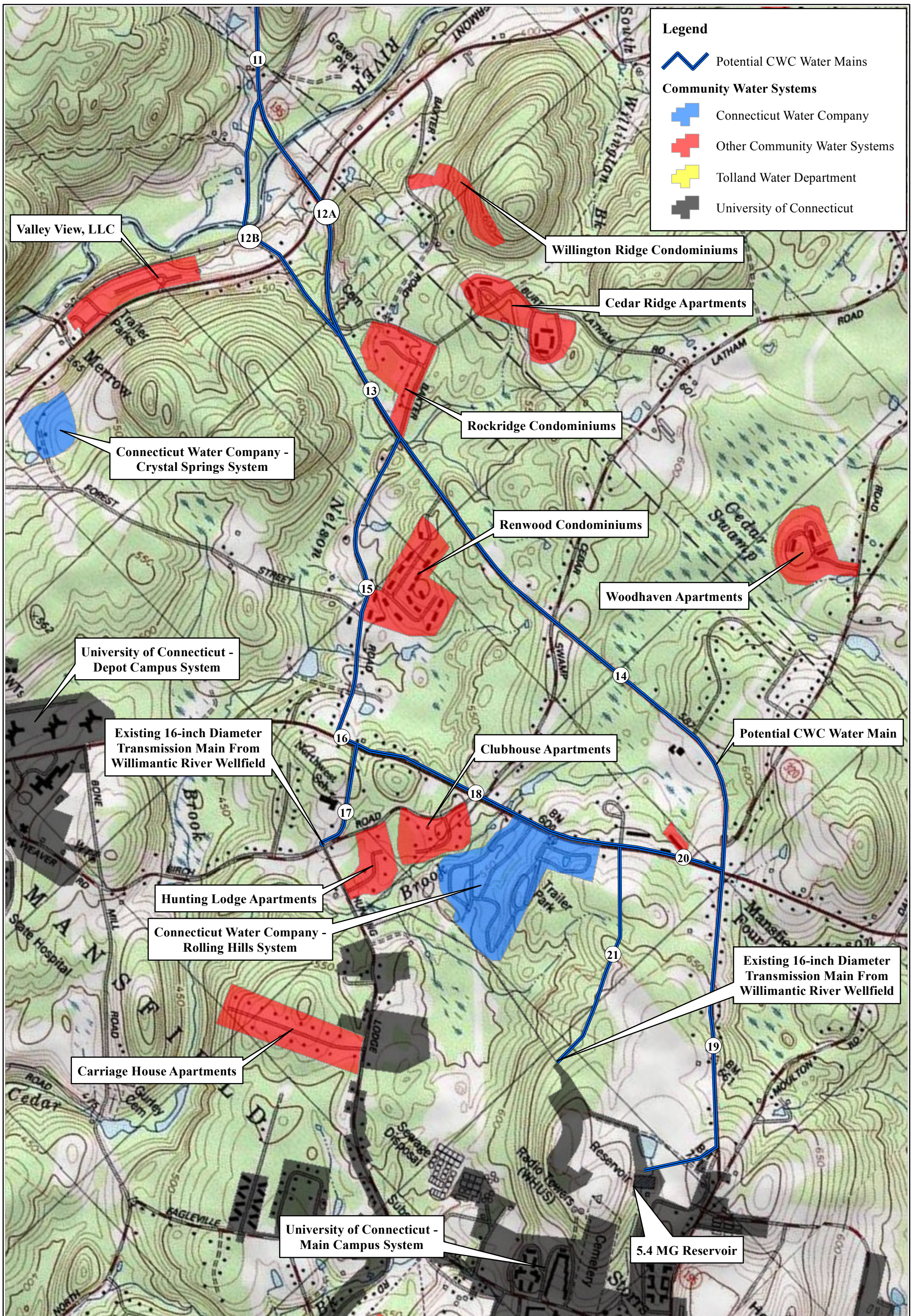
Figure 3.4-2: Mansfield Section of CWC Interconnection Alternative
