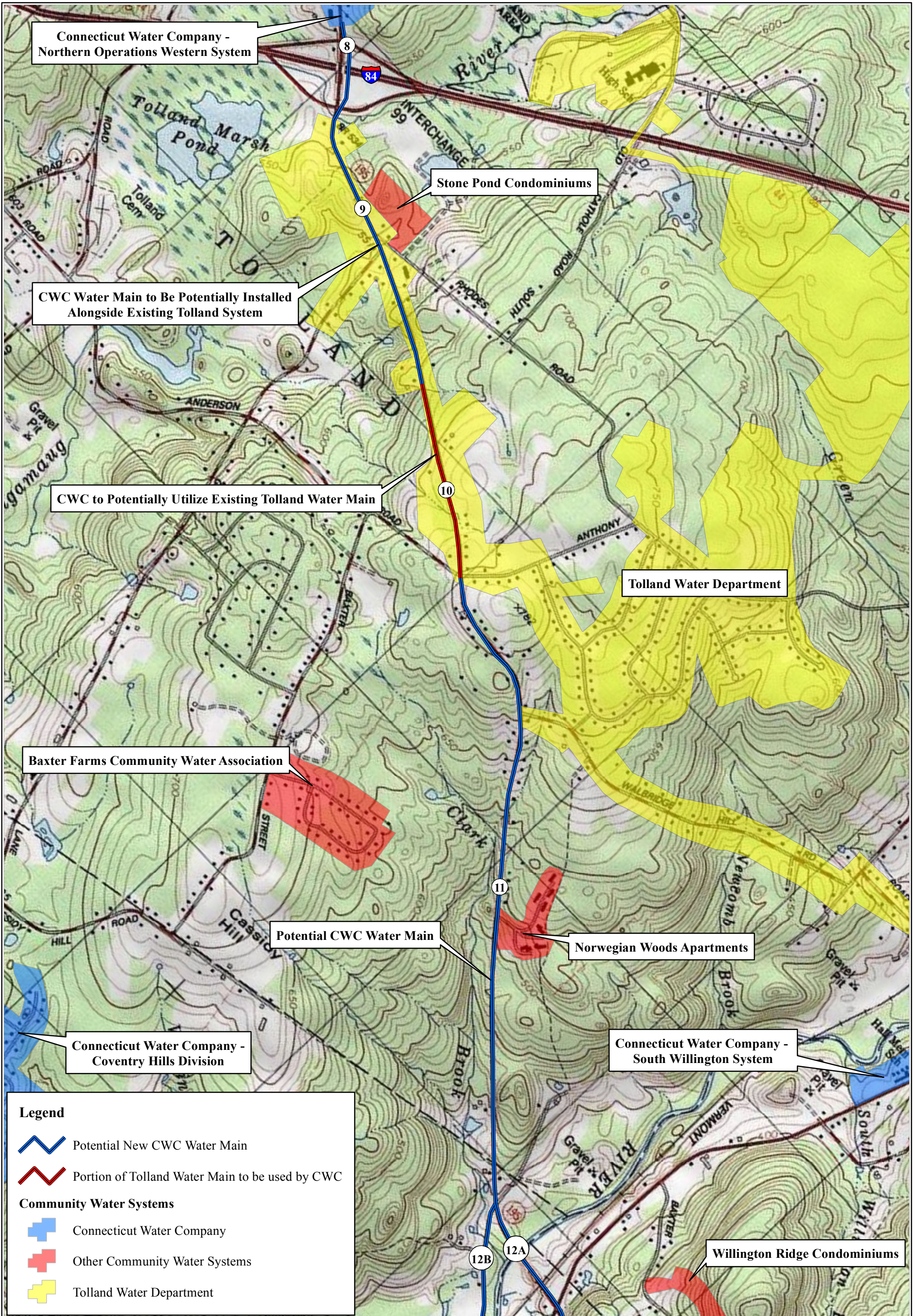
Figure 3.4-1: Tolland Section of CWC Interconnection Alternative
