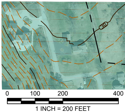
FIGURE 3-1 TOPOGRAPHY, GEOLOGY AND SOILS Seaside State Park Master Plan ENVIRONMENTAL IMPACT EVALUATION May 2017
