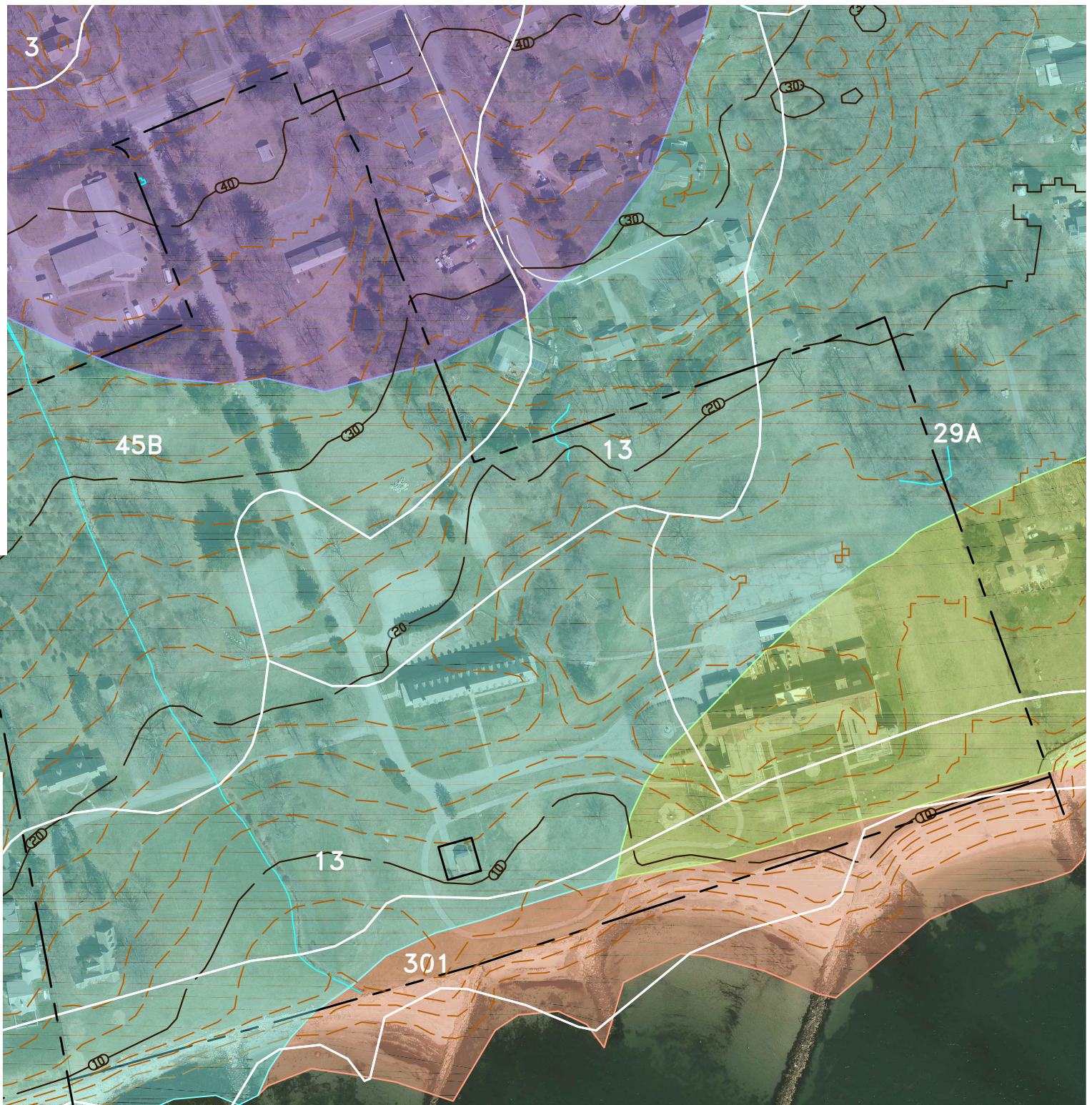
FIGURE 3-1 TOPOGRAPHY, GEOLOGY AND SOILS Seaside State Park Master Plan ENVIRONMENTAL IMPACT EVALUATION May 2017
