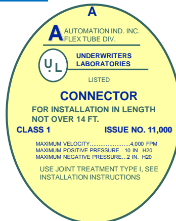
Flexible Air Connector Label Representation
