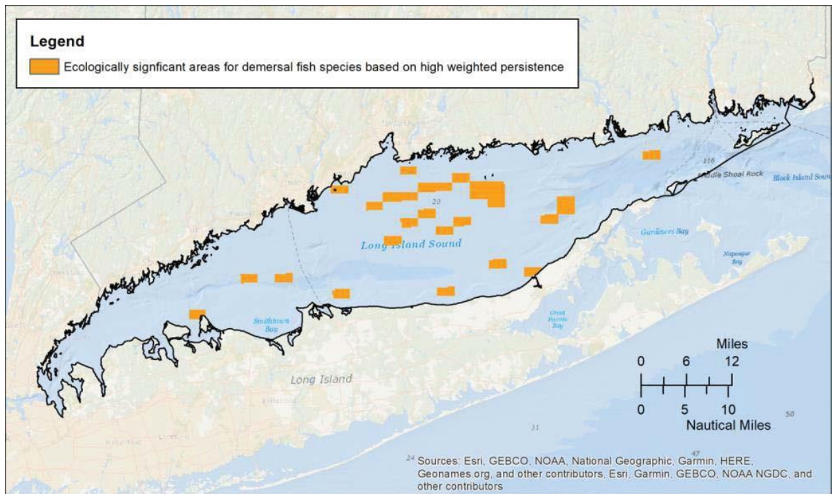
Figure 3-21 A map showing one component of Ecologically significant areas for fish: areas of high weighted persistence for demersal fish subgroups based on TNC's LISEA.
