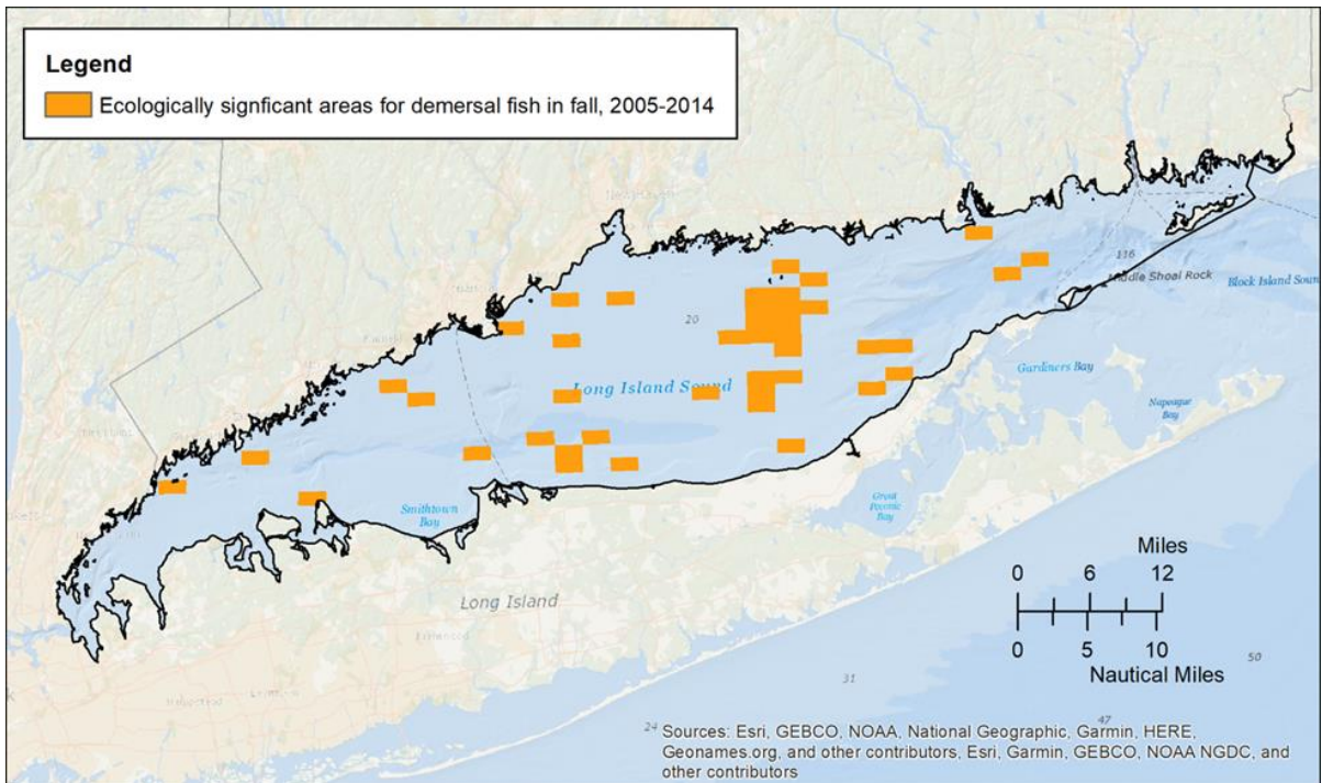
Figure 3-25 A map showing one component of Ecologically Significant Areas for fish: the top quintile of demersal fish species abundance in fall from LISTS 2005-2014.
