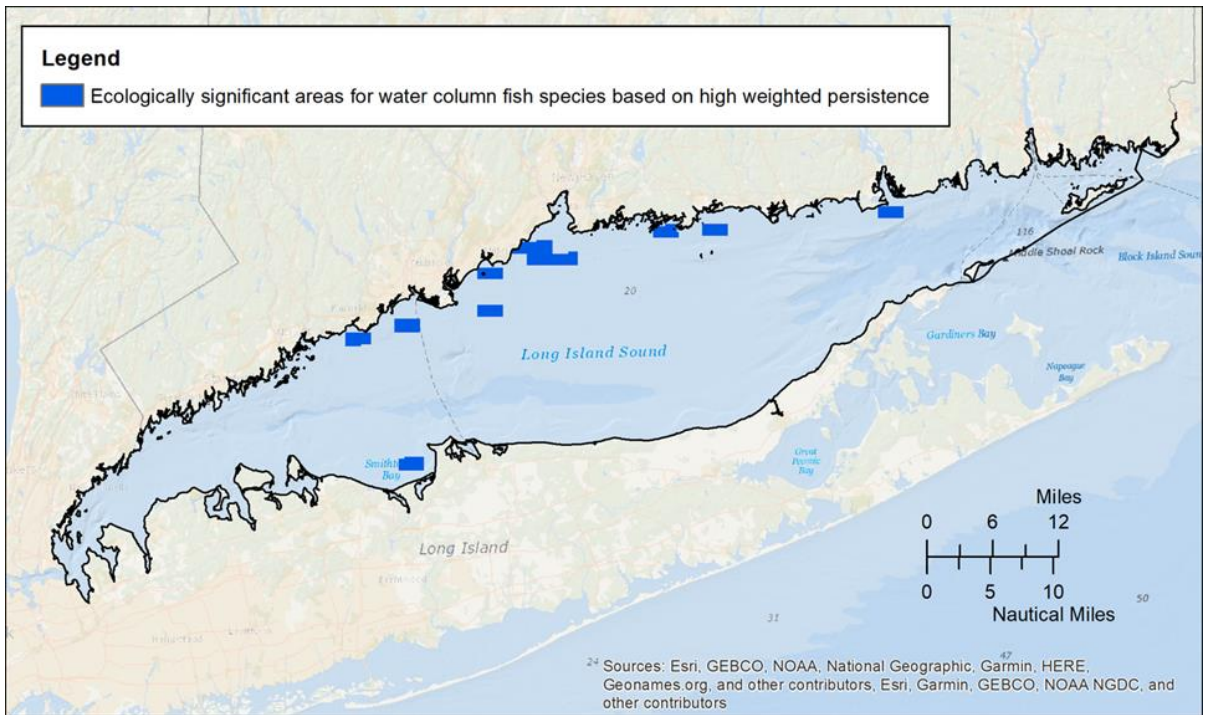
Figure 3-22 A map showing one component of Ecologically Significant Areas for fish: areas of high weighted persistence for water column (pelagic and diadromous) fish subgroups based on TNC's LISEA.
