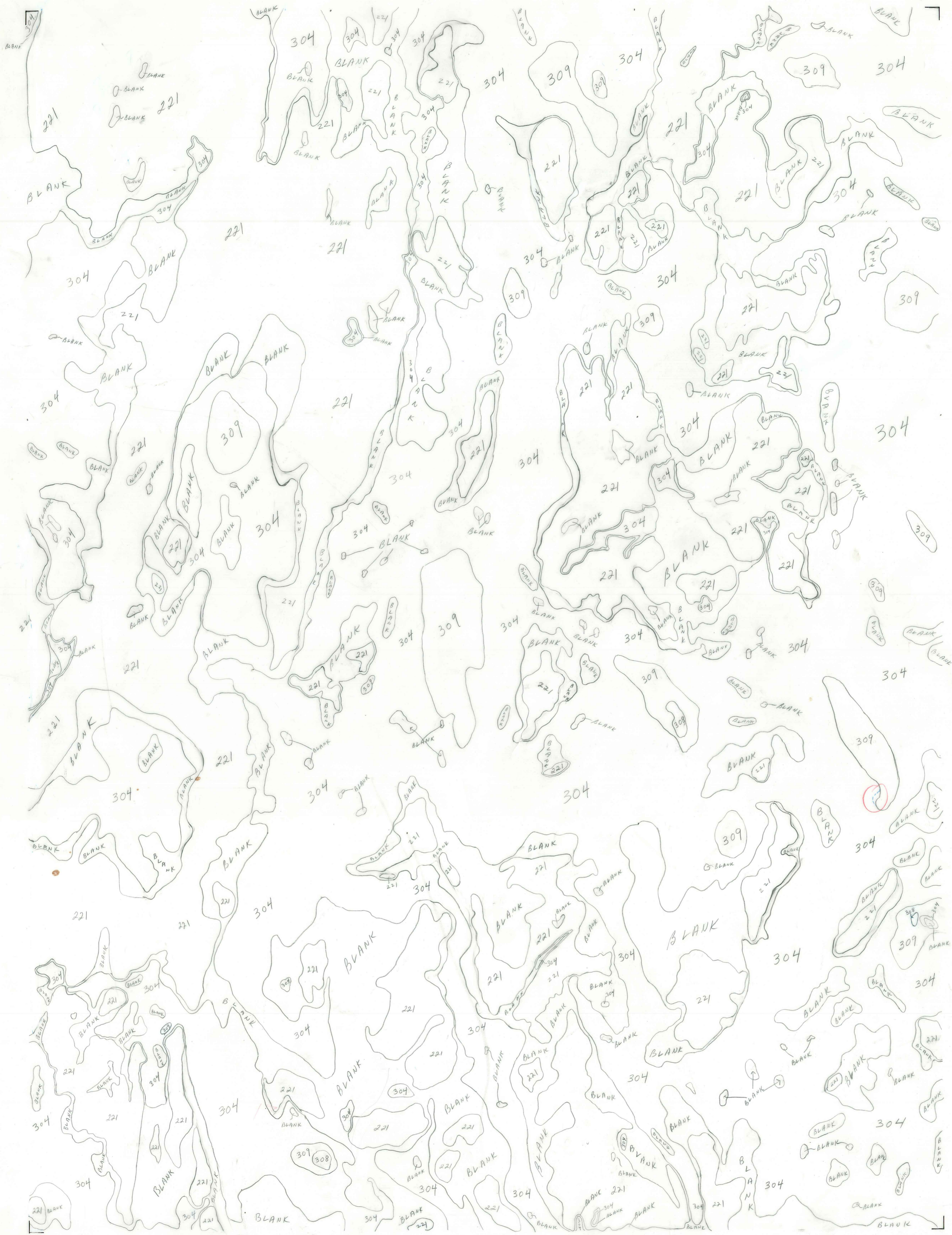
Depth to Bedrock Marlborough Quadrangle, Connecticut
