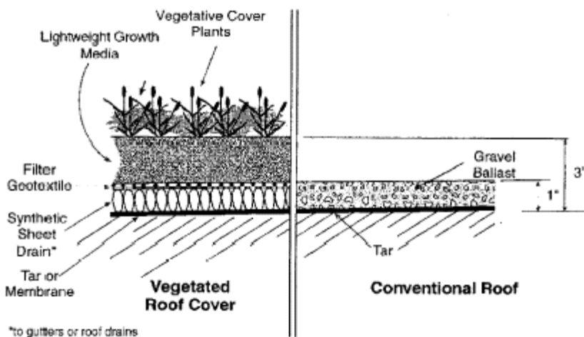
Figure 4.19 – Example Vegetated Rooftop Cross-section
