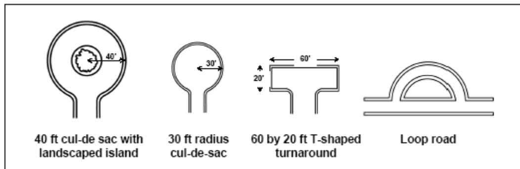
Figure 4.4– Different styles of turnarounds. Source: Adapted from Atlanta Regional Commission, 2001.
