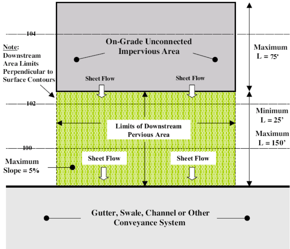
Figure 4.13– Standards for disconnecting impervious surface via sheet flow. Source: New Jersey Department of Environmental Protection, 2004.
