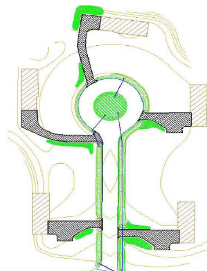
Figure 3.7 – Cul-de-sac designs.
