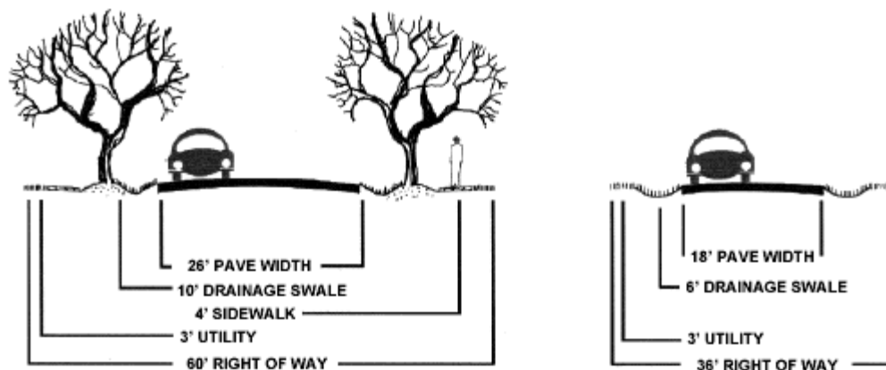
Figure 4.6 – Reduced road widths. Source: Atlanta Regional Commission, 2001.
