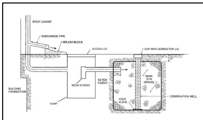
Figure 4.21 – Schematic of a drywell with optional sump to facilitate cleanout. Source: Adapted from New York, 2001.
