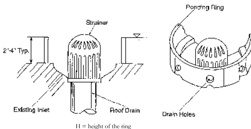
Figure 4.18 – Roof ponding rings. Source: Tourbier, 1974.
