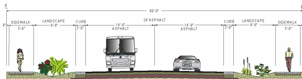
Figure 3.4. Open section roadways.
