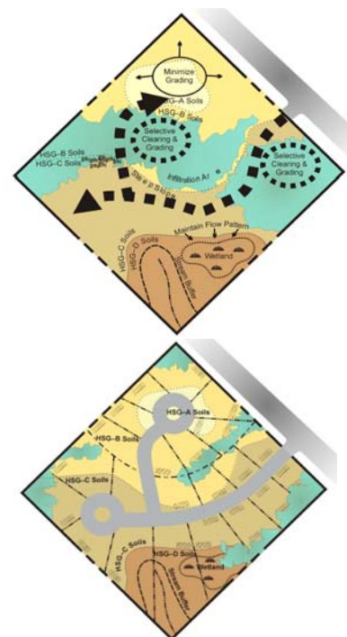
Figure 2.5 – Optimizing the use of green space.
