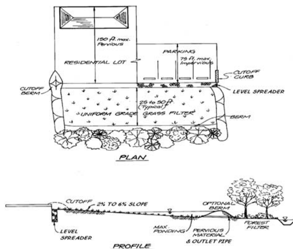
Figure 4.15 – Drawing of a vegetative filter strip. Source: Atlanta Regional Commission, 2001.
