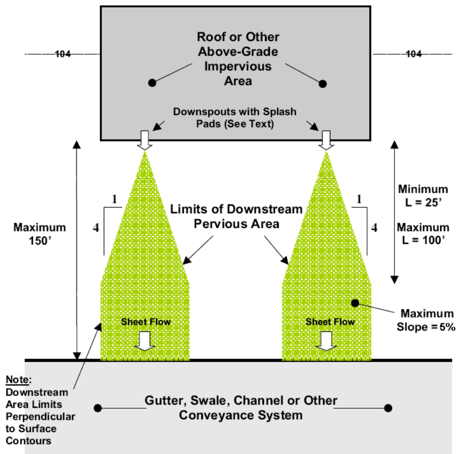
Figure 4.14 – Standards for disconnecting impervious surface via downspouts. Source: New Jersey Department of Environmental Protection, 2004.
