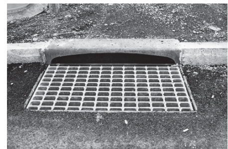
Figure 25. Bike Friendly Catch Basin Grate
