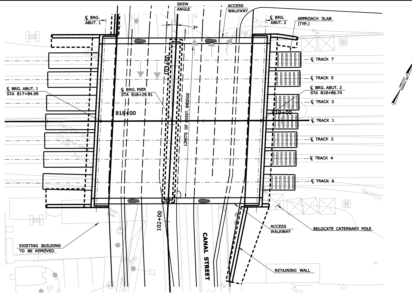
PROPOSED PLAN SCALE: 1" = 30'
