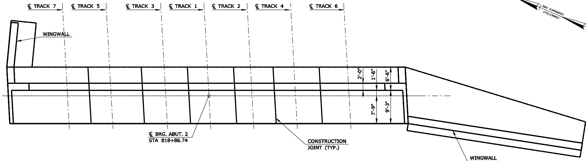
ABUTMENT 2 PLAN SCALE: 1/16" = 1'-0"
