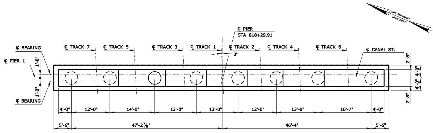
PIER PLAN SCALE: 1/16" = 1'-0"
