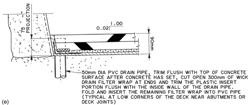
FIGURE 8 Examples of details provided in standard drawings: (a) Composite deck, (b) Noncomposite deck, (c) Detail A, (d) Legend, (e) Drain pipe detail [Source: Alberta Transportation].
