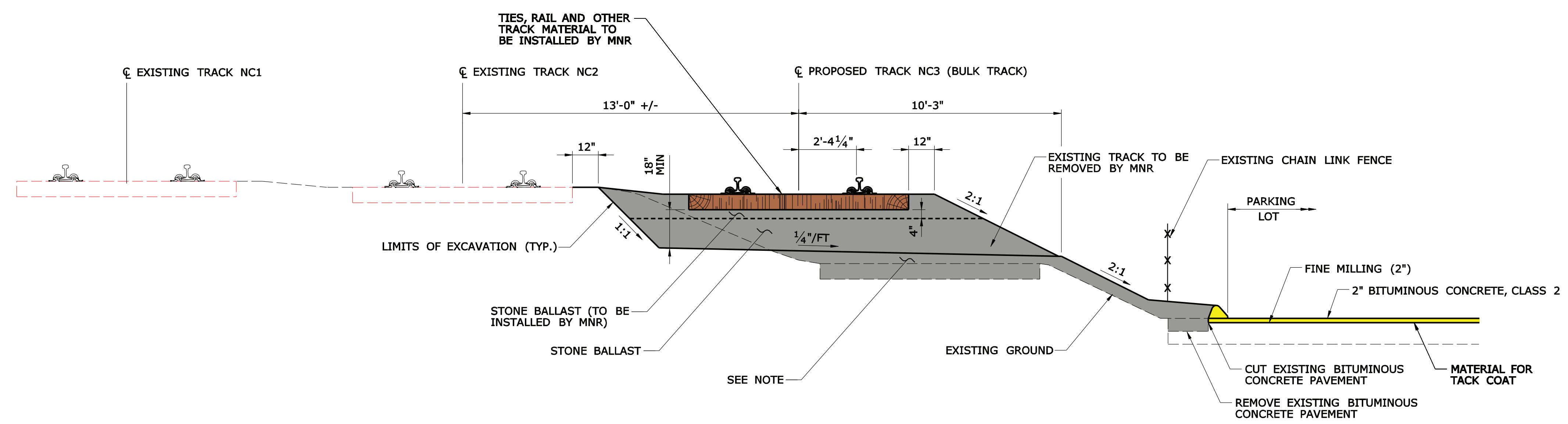
TRACK NC3 (BULK TRACK) TYPICAL SECTION 1
