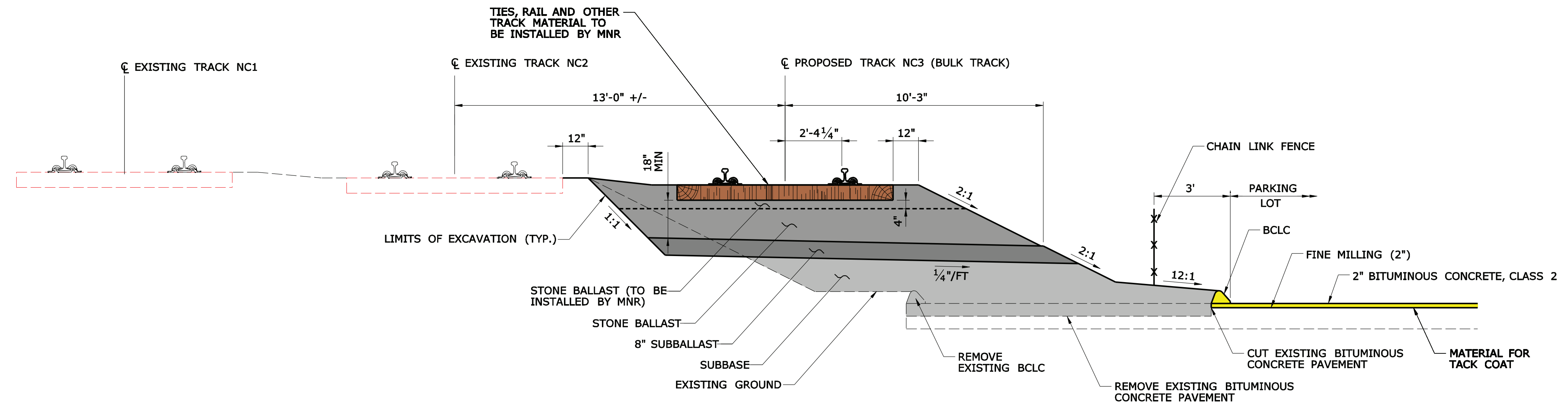
TRACK NC3 (BULK TRACK) TYPICAL SECTION 2
