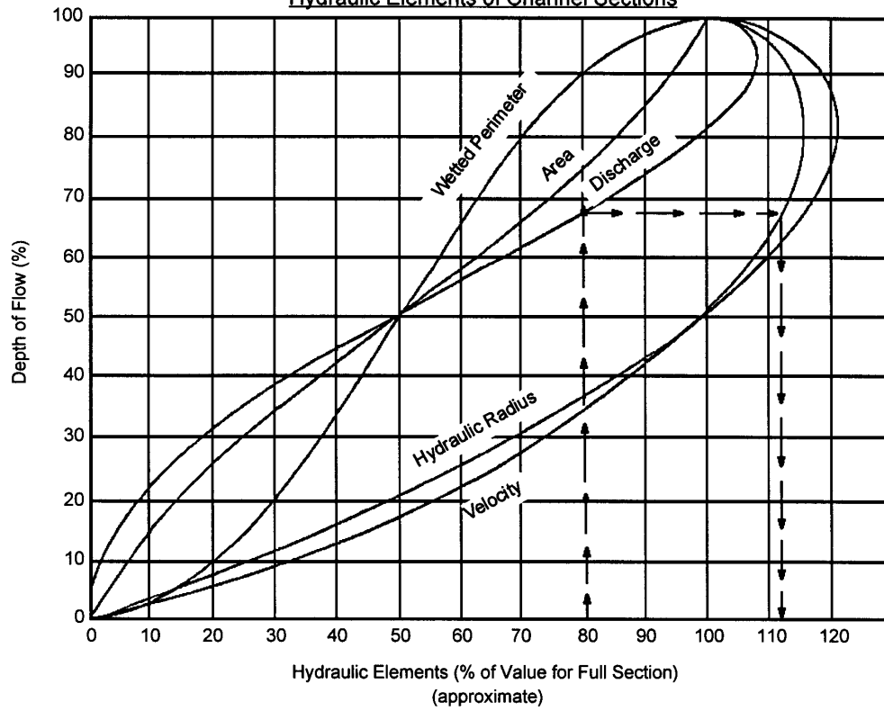
Figure 11-11 Values Of Hydraulic Elements Of Circular Section For Various Depths Of Flow – Metric or English units
