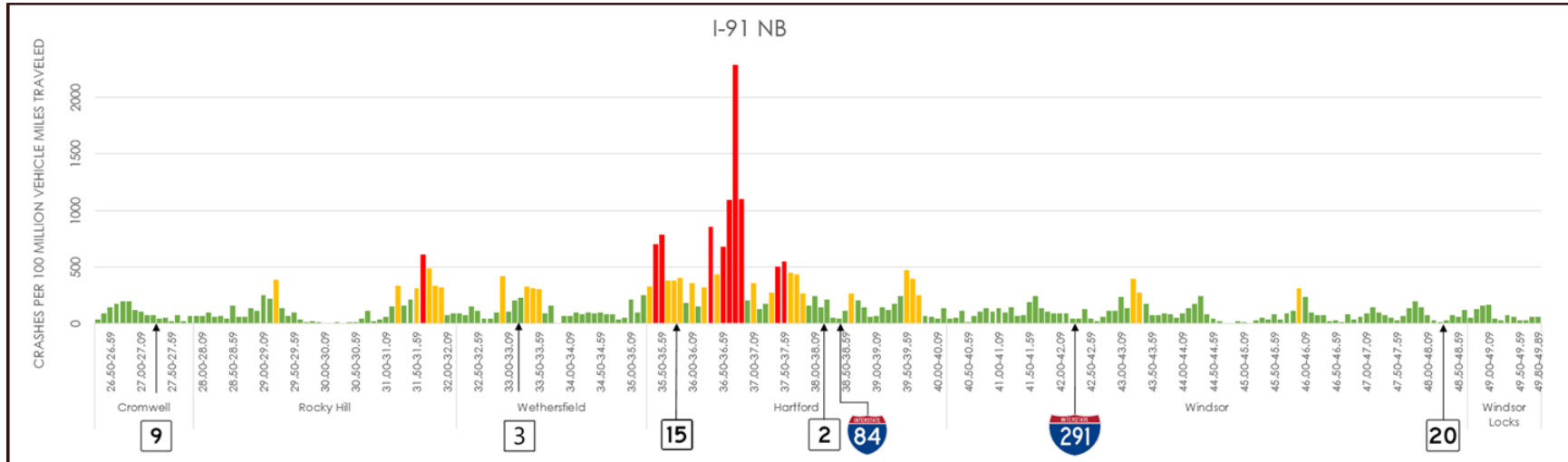
Figure 3-12: I-91 Northbound Crash Rates
