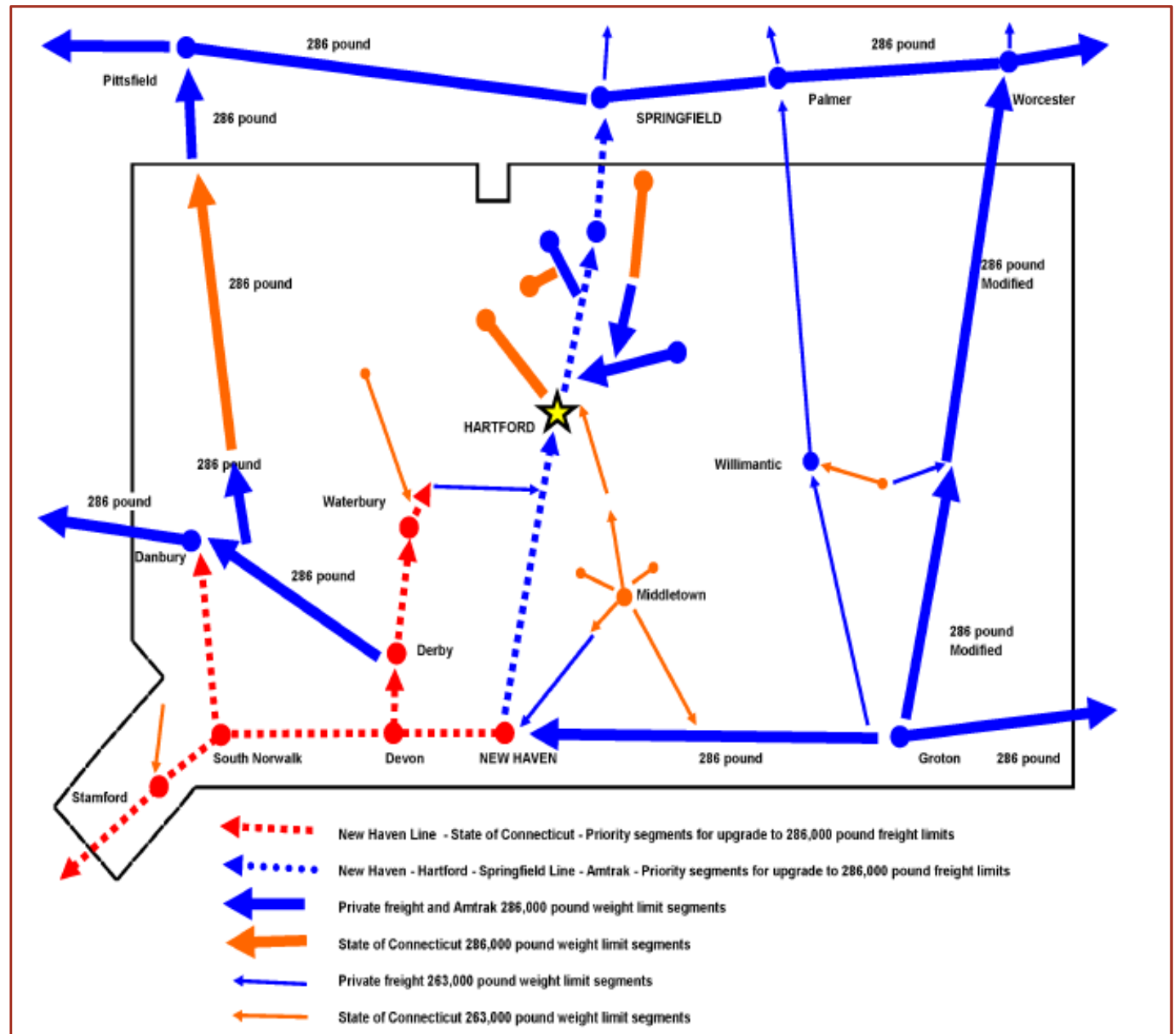
Figure 5-7: Freight Rail 286K Upgrade Prioritization (2012 State Rail Plan)
