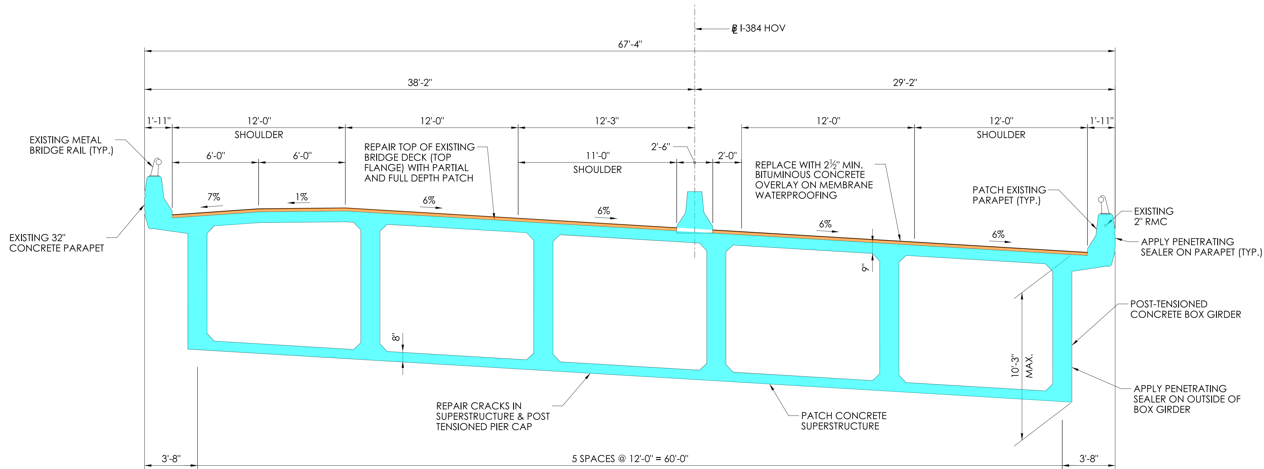
BRIDGE 05685 TYPICAL SECTION (LITTLE FOOT) SCALE: 1/4" = 1'-0"
