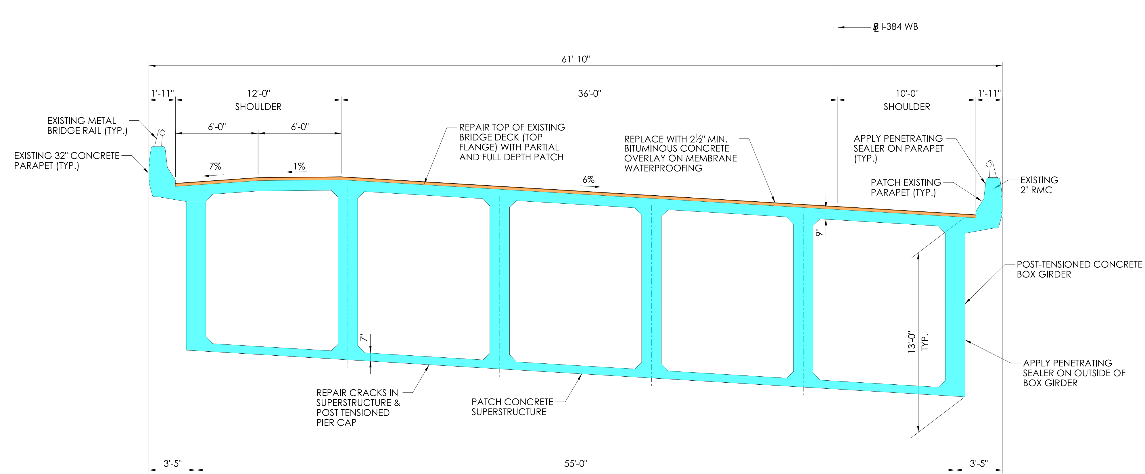
BRIDGE 05686 TYPICAL SECTION (BIG FOOT) SCALE: ¼" = 1'-0"
