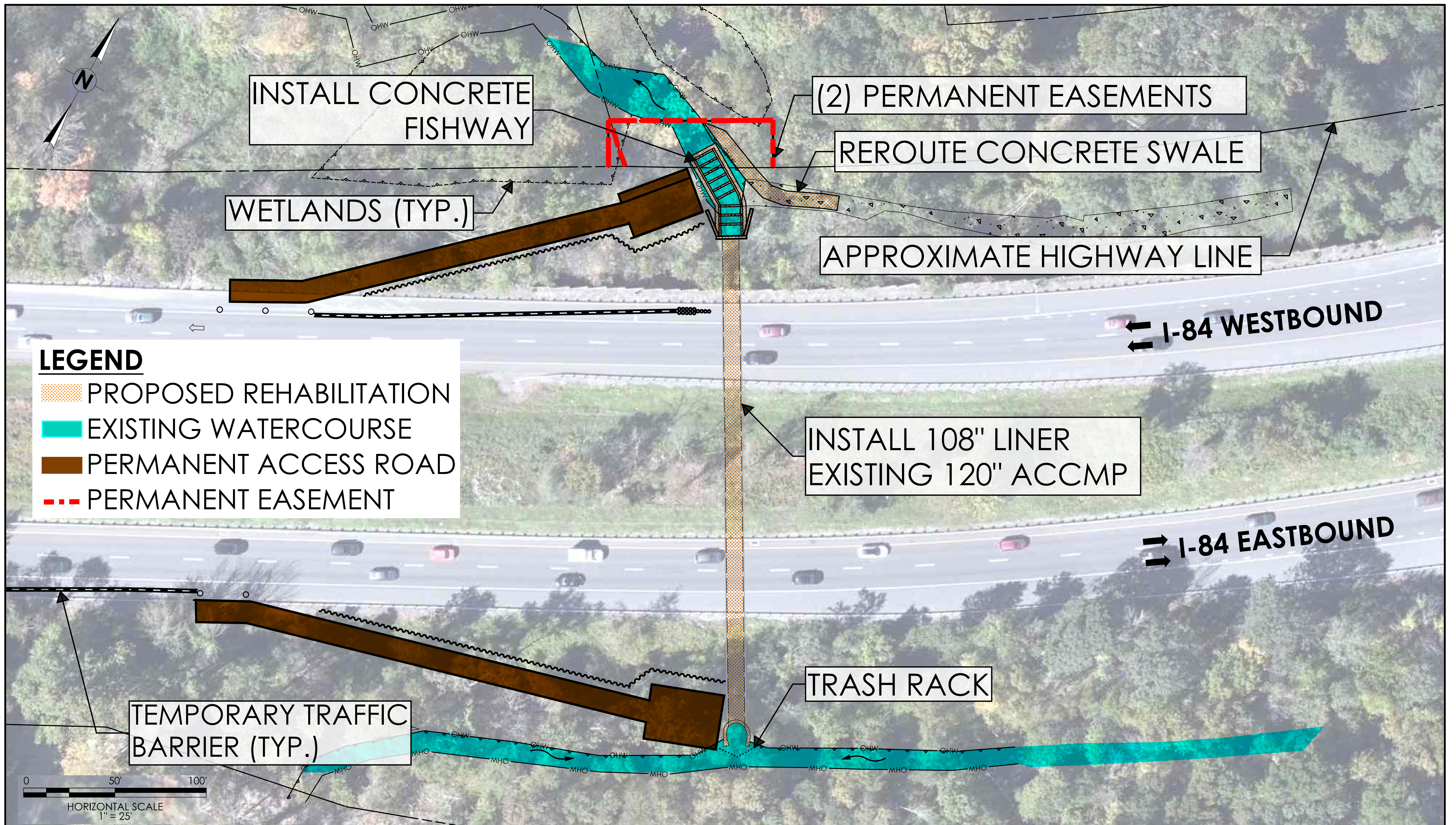
BRIDGE NO. 07044 - GENERAL PLAN INTERSTATE 84 OVER OLIVER BROOK SOUTHURY, CONNECTICUT
