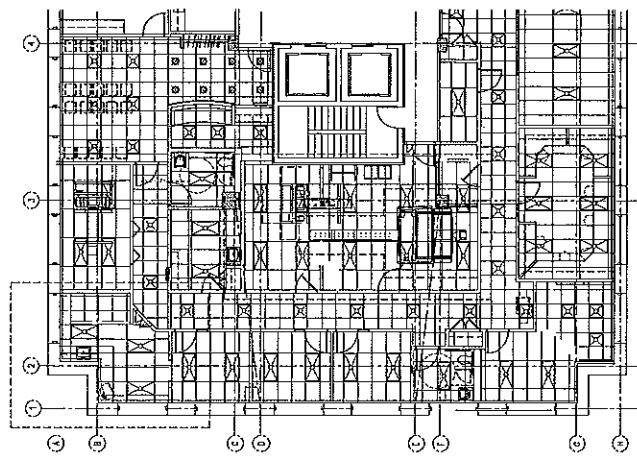
3 RCP 8TH FLOOR A1.02/1/8"=1'-0"
